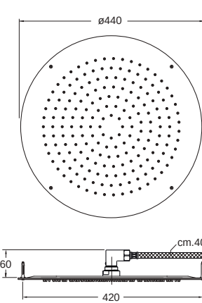
CRIPD361 51 chrome 13 black matt 34P PVD brushed rose gold 46P PVD polished rose gold 55P PVD infinity black 56P PVD polished gold brass 72 polished black chrome 75 brushed black chrome 76 imperial black 96P PVD brushed gold brass
